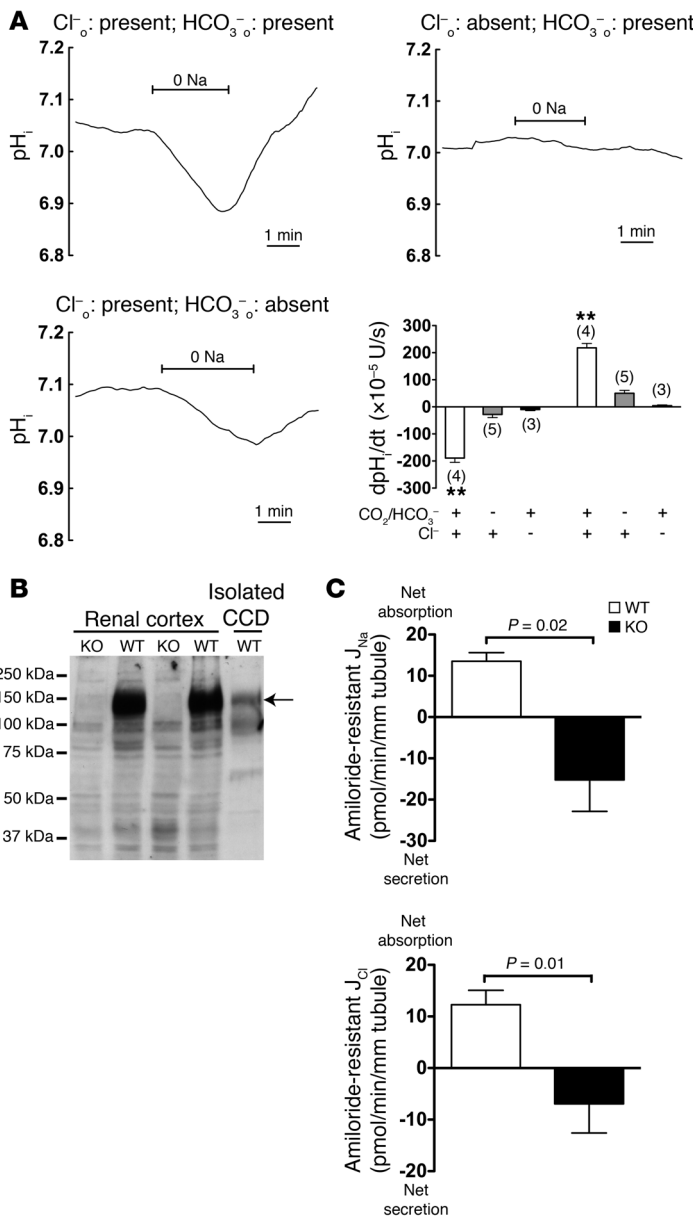
Figure 6 Detection and functional characterization of NDCBE in collecting ducts isolated from wild-type mice fed a Na + -depleted diet. (A) Na + dependence of \text{pH}_i changes in intercalated cells of CCDs isolated from mice fed a Na + -depleted diet. Traces are the average of \text{pH}_i changes recorded when luminal Na + was removed from, and then readded to the perfusate. Upper-left panel: Both \text{Cl}^- and \text{HCO}_3^-/\text{CO}_2 were present in the extracellular fluid; mean starting \text{pH}_i (immediately before luminal Na + removal) was 7.03 \pm 0.04 . Upper right: extracellular \text{Cl}^- was absent; mean starting \text{pH}_i was 7.03 \pm 0.05 . Lower left: extracellular \text{HCO}_3^-/\text{CO}_2 was absent; mean starting \text{pH}_i was 7.09 \pm 0.11 . Lower right: initial rates of \text{pH}_i changes during exposure to different solutions. Values are mean \pm SEM, with number of tubules in parentheses. Statistical significance was tested by ANOVA followed by Bonferroni's post-hoc test. ** P < 0.01 versus all other groups. o, outside. (B) Western blot analyses of NDCBE in the mouse kidney and CCD. Western blot analyses of 50 \mu\text{g} membrane fraction proteins from renal cortex isolated from Ndcbe -/- mice or wild-type mice or of proteins from 100 CCDs (corresponding to ~25 mm of tubule) isolated from wild-type mice. NDCBE was detected in the renal cortex or isolated tubules of wild-type but not of Ndcbe -/- mice. Note that the apparent difference in abundance of NDCBE between the lane loaded with total cortex and the one loaded with isolated CCD does not reflect an enrichment of the cortex versus the CCD, but actually only reflects the difference in the quantity of protein loaded. (C) Analyses of amiloride-resistant Na + and Cl - transepithelial fluxes in CCDs isolated from NDCBE-KO mice maintained on a Na + -depleted diet. Fluxes were measured in the presence of 10 -5 M amiloride in the perfusate to reflect only the amiloride-resistant, HCTZ-sensitive component of NaCl reabsorption. Values are mean \pm SEM; statistical significance was assessed by unpaired Student's t test with Welch's correction, when appropriate. n = 5 in each group.
