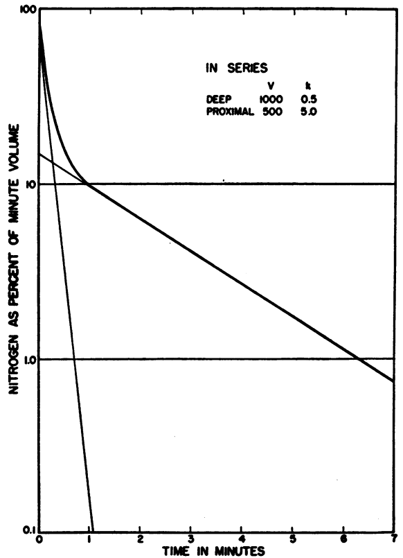
FIG. 4. THEORETICAL RATES OF NITROGEN ELIMINATION FROM THE SAME TWO SPACES AS IN FIGURE 2 BUT ARRANGED SO THAT ALL OF THE AIR VENTILATING THE DEEP SPACE PASSES THROUGH THE PROXIMAL SPACE
